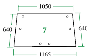
26/4072-14 (D.6772, 930-174) Trasero (superior, 6 agujeros) Rear (Upper, 6 holes)
