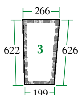
26/4015-2 (D.7042, AL.27352) Delantera (izq.) Front (LH)
