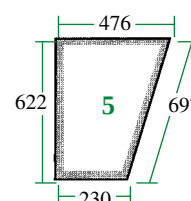
26/4032-1 (D.6769, AL.27356) Puerta (inferior izq.) Door (Lower LH)
