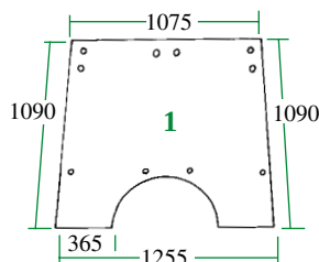
26/4000-39 (D.8056, L.59466) (003482 ⇨) Parabrisas Windscreen
