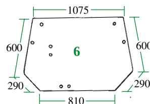
26/4072-29 (D.8051, L.57284) Trasero (superior) Rear (Upper)
