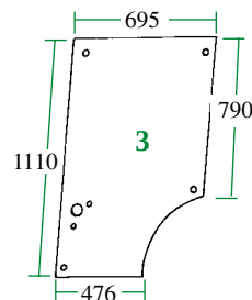
26/4022-23 (D.8054/A, L.57904) (3 cil./cyl.) Puerta (izq. o drcha. superior) Door (Upper LH or RH)
