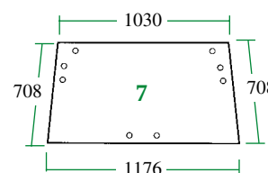
26/4072-28 (D.8025, L.36075) Trasero (superior, 8 agujeros) Rear (Upper, 8 holes)
