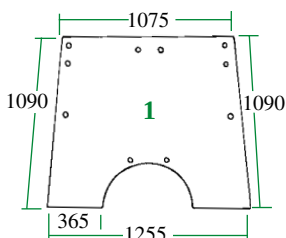
26/4000-38 (D.8053, L.57290) (⇨ 003481) Parabrisas Windscreen
