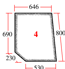
25/4034-1 (D.7043, 3125458R1) Porte (haut droit) Door (RH upper)
