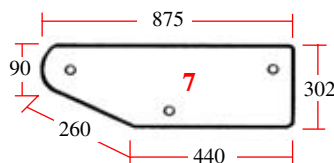
25/4073-21 (D7065, 1535071C1) Arrière (bas) Rear (lower)
