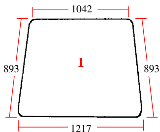
25/4000-36 (D.7010, 3233045R1) Pare-brise Windscreen
