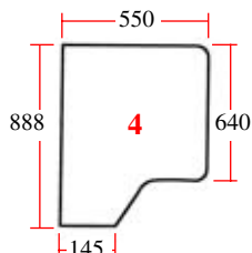
25/4027-2 (D.7014, 3233051R1) Porte (fixe) Door
