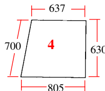
20/4028-2 (D7025, K303700) Porte (droite) Door (RH)
