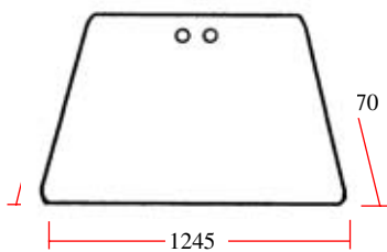
25/4000-48 (D.7090, 144768A1) Pare-brise 2 trous Windscreen 2 holes
